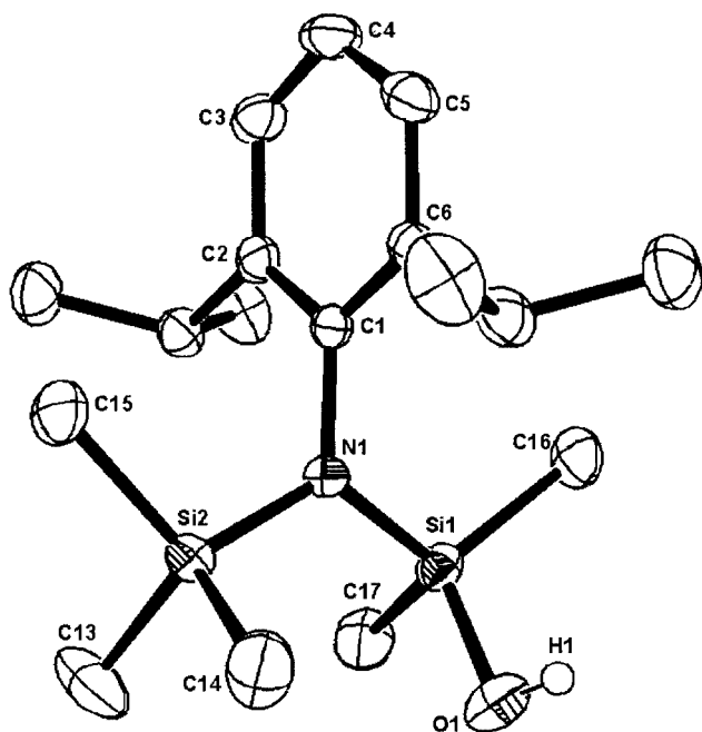
Figure 2. ORTEP diagram of 2c shown at the 50% probability level. All the hydrogen atoms have been omitted except those of the hydroxy group.
