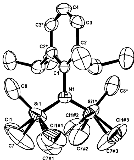
Figure 1. ORTEP diagram of 1c shown at the 50% probability level. All the hydrogen atoms are omitted for clarity.
