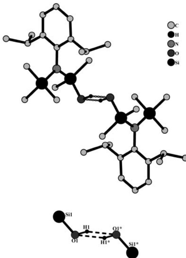
Figure 3. (Top). Formation of a cyclic dimer due to intermolecular hydrogen bonding between two silanol molecules. (Bottom). A perfectly planar arrangement of the four-membered O 2 H 2 ring. The metric parameters are: O1–H1, 0.840(1) Å; H1...O1*, 2.057(1) Å; O...O*, 2.857(2) Å; O–H...O*, 158.94(9)°; symmetry, 1 – x , 1 – y , 2 – z .
