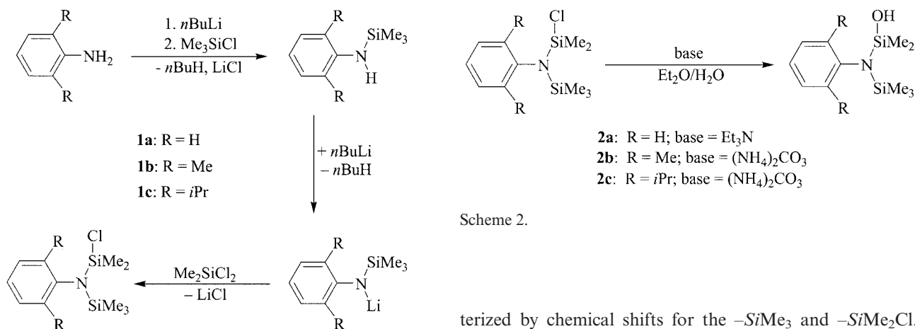
Scheme 1.
